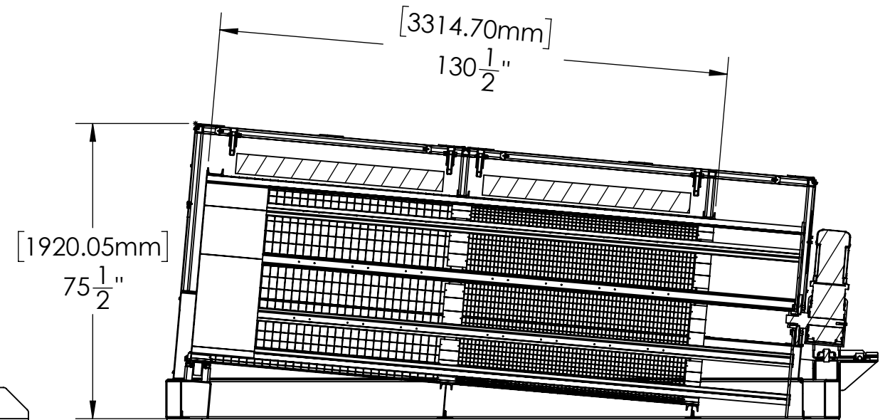
SECTION B-B
