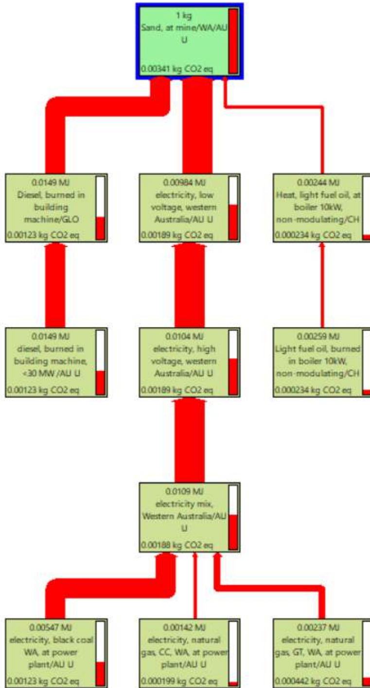
Figure 2.2: Breakdown of embodied GHG emission factor of virgin (natural) sand
