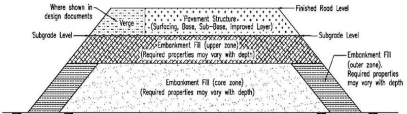
Figure 3.3: Embankment zones
