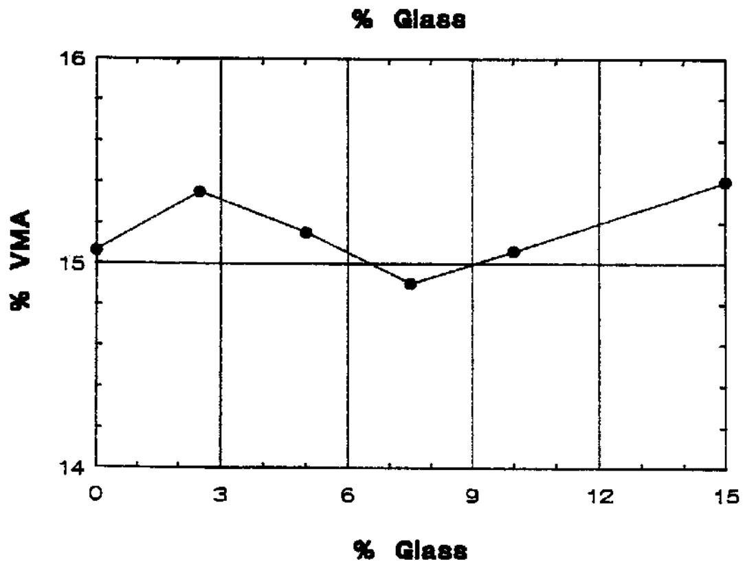
FIGURE 6. Influence of Crushed Glass Content on % Air Voids and % VMA for AC5 Grade Asphalt.
