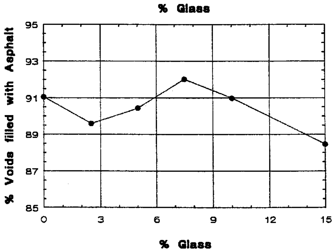
FIGURE 5. Influence of Crushed Glass Content on Unit Weight and % Voids filled with Asphalt for AC5 Grade Asphalt.
