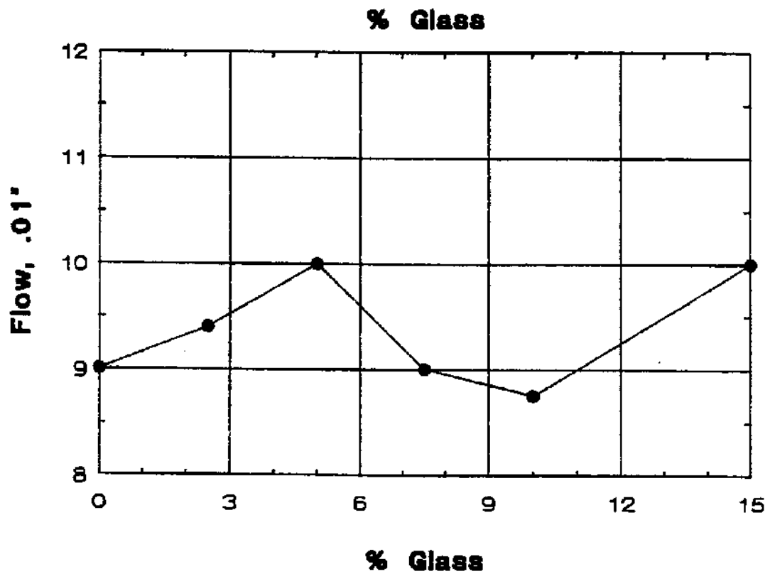
FIGURE 1. Influence of Crushed Glass Content on Stability and Flow for AC2.5 Grade Asphalt.
